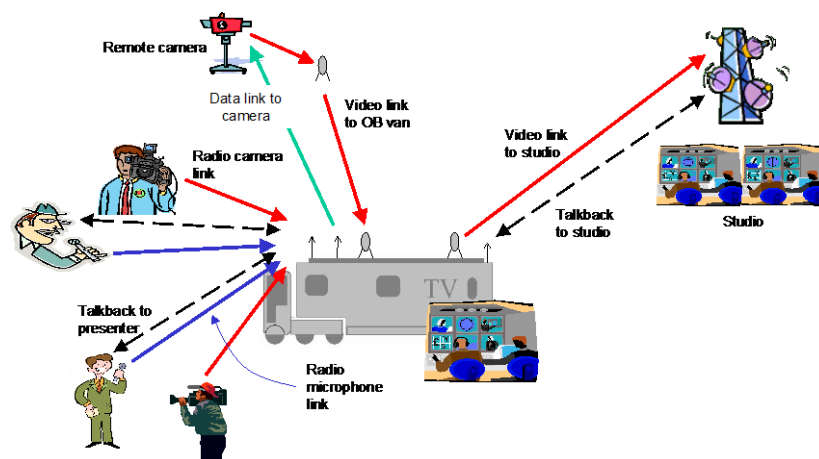
Figure 12-1: Use of spectrum in an outside broadcast
