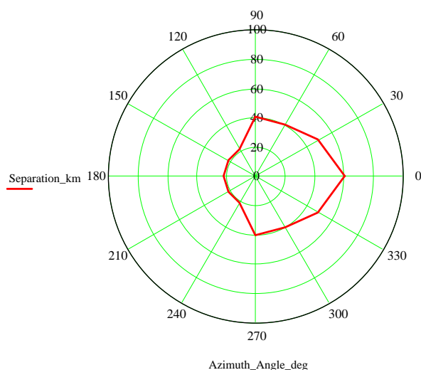
Figure 23: Separation Distances (NGMB BS Interference into Digital/Analogue MMDS Receiver at 5 m Height)
