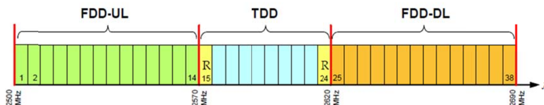
Figure 12: 2.6 GHz Band Plan (Ref: ECC Report 131)
