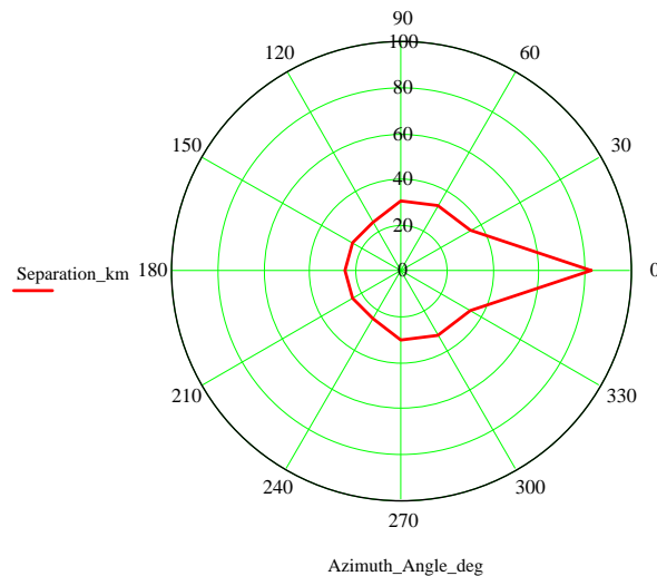
Figure 24: Separation Distances (NGMB BS Interference into Digital/Analogue MMDS Parabolic Receiver)
