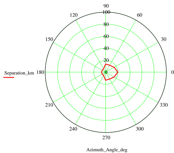
Figure 22: Separation Distances (NGMB Pico BS Interference into Digital/Analogue MMDS Receiver)
