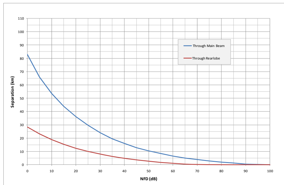
Figure 27: Variation of Separation Distance with NFD (NGMB BS Interference into Digital/Analogue MMDS Receiver)
