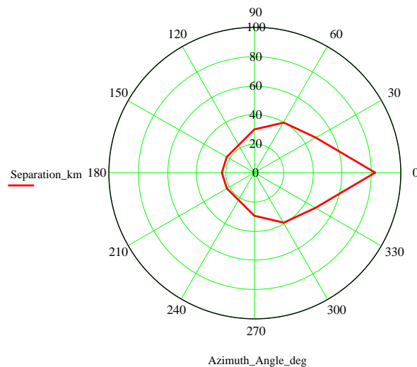
Figure 25: Separation Distances (NGMB BS Interference into Digital/Analogue MMDS Planar Receiver)
