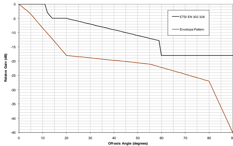
Figure 17: MMDS Transmitter Antenna Elevation Patterns
