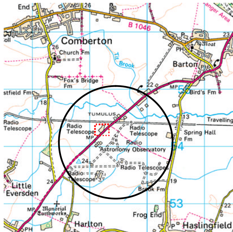
Figure B6: Cambridge area (1 km range indicated, showing local buildings at ~500 m from telescopes)
