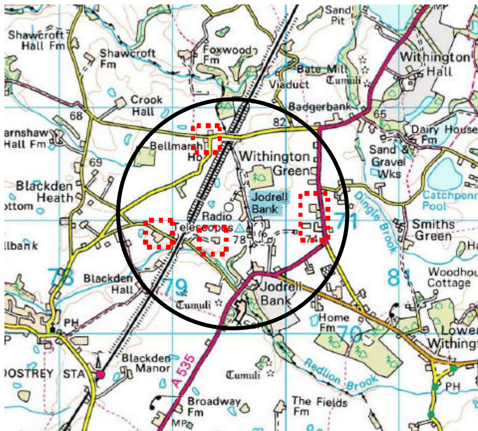
Figure B1: Jodrell area (1 km range indicated, showing local housing at ~500 m from telescopes)
