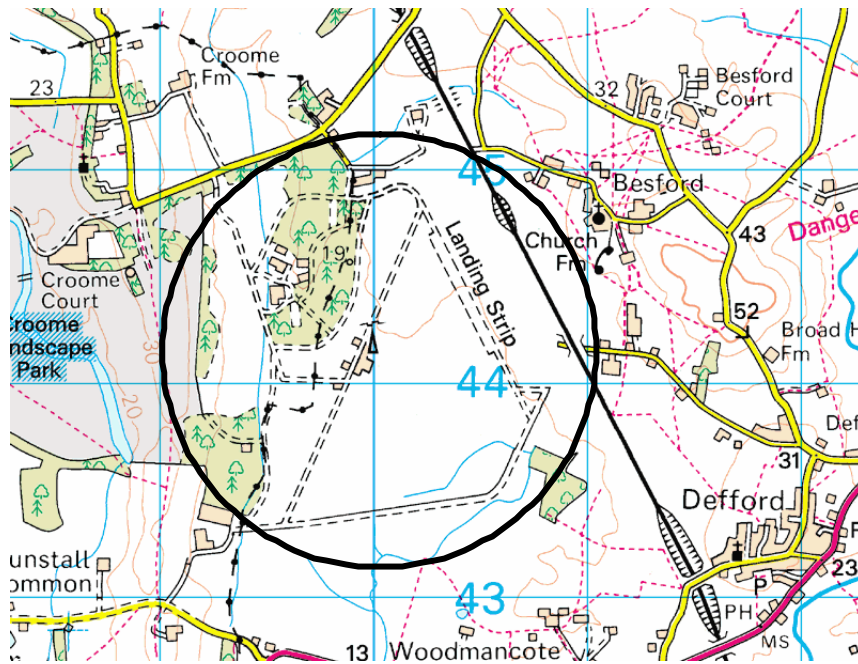
Figure B2: Defford area (1 km range indicated)
