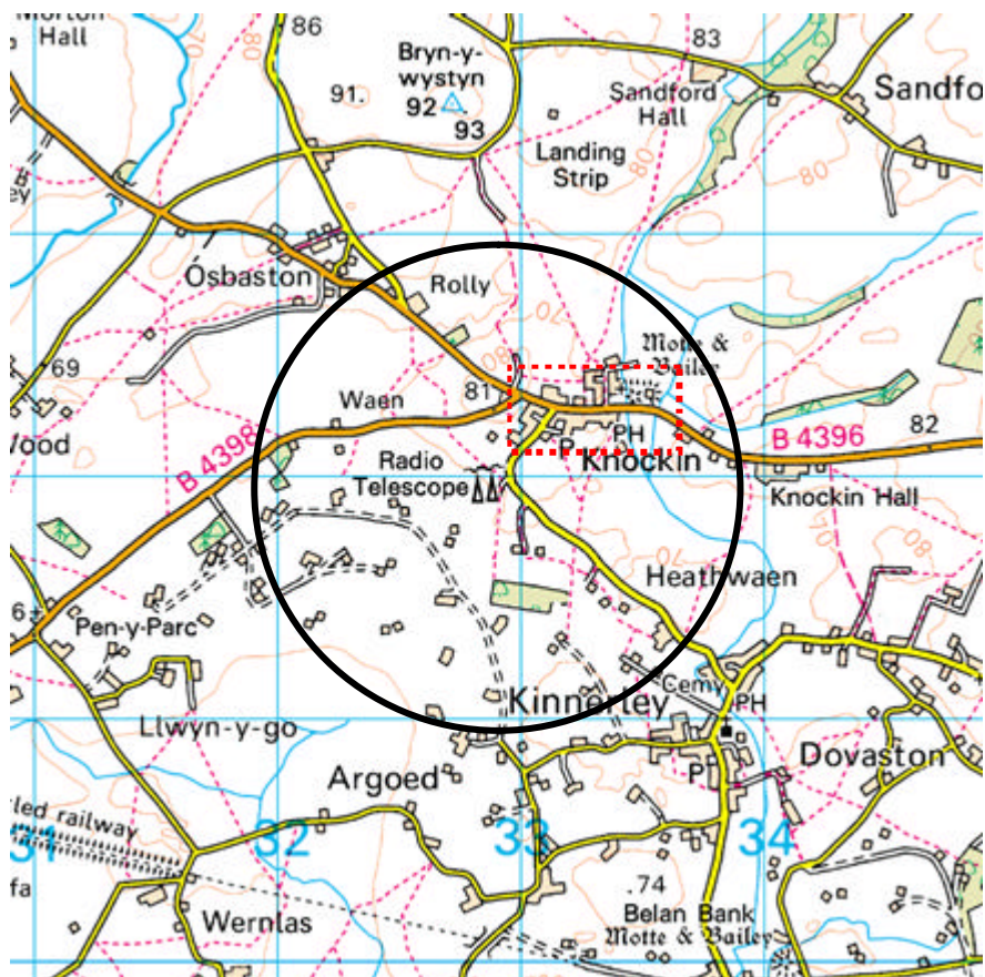
Figure B3: Knockin area (1 km range indicated, showing local housing at ~500 m from telescopes)
