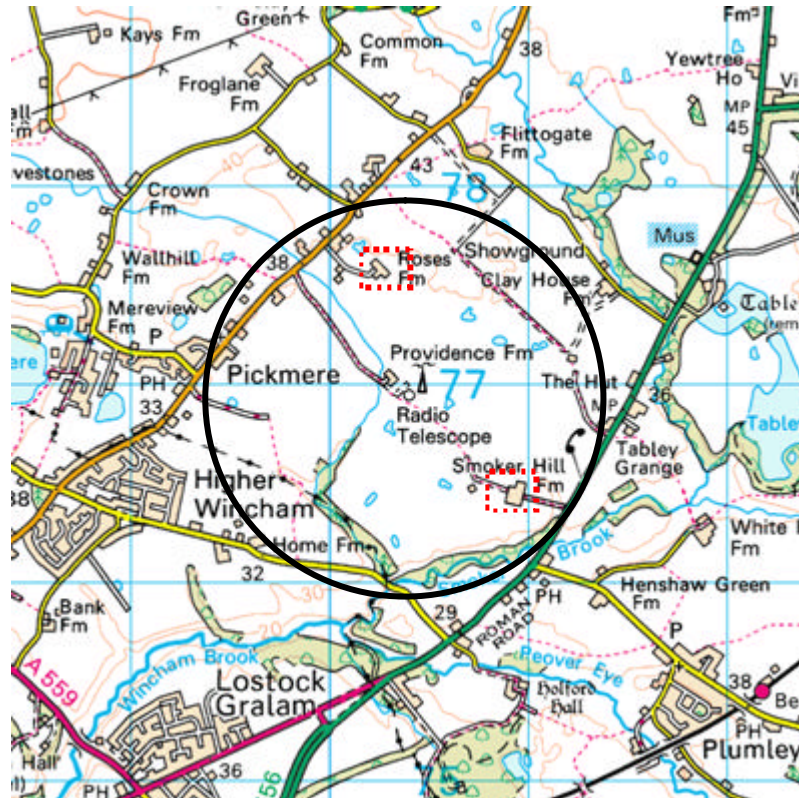
Figure B4: Pickmere area (1 km range indicated, showing local farms at ~500 m from telescopes)
