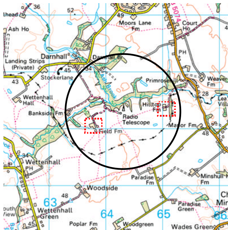
Figure B5: Darnhall area (1 km range indicated, showing local farms at ~500 m from telescopes)
